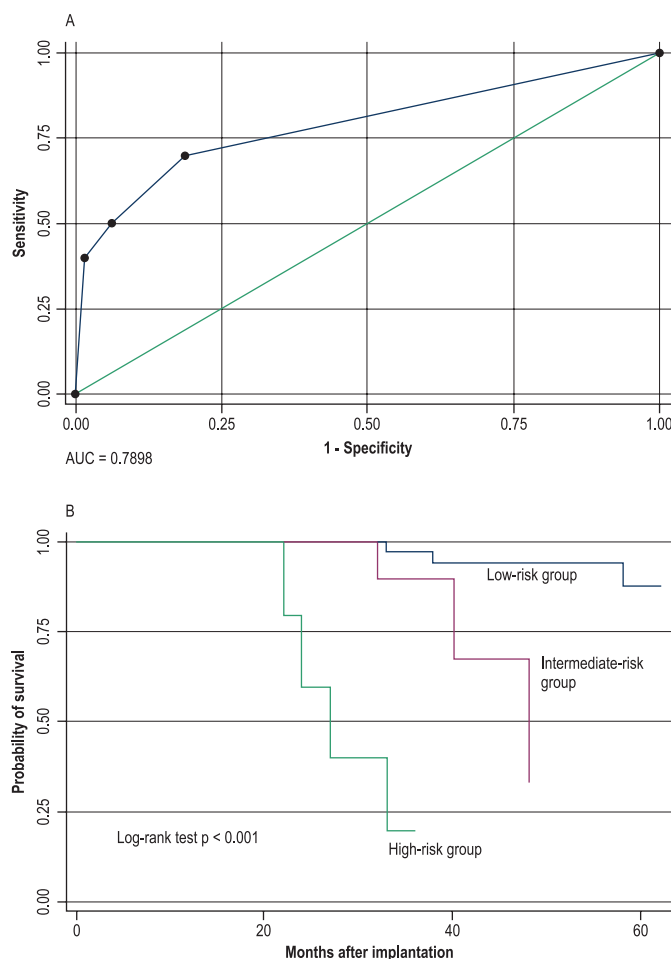
Figure 3 – A: ROC curve of the model at time 3 (2nd year), with the variables right ventricle (RV) dysfunction and functional class (FC) III and IV compared with I and II, with an area under the curve (AUC) of 0.789, sensitivity of 40%, specificity of 98.4% and accuracy of 90.5%. B: Kaplan-Meier curve showing that the absence of the variables RV dysfunction and FC III / IV (Class A - low risk) indicates an event-free rate of 97.5% at 30 months.
